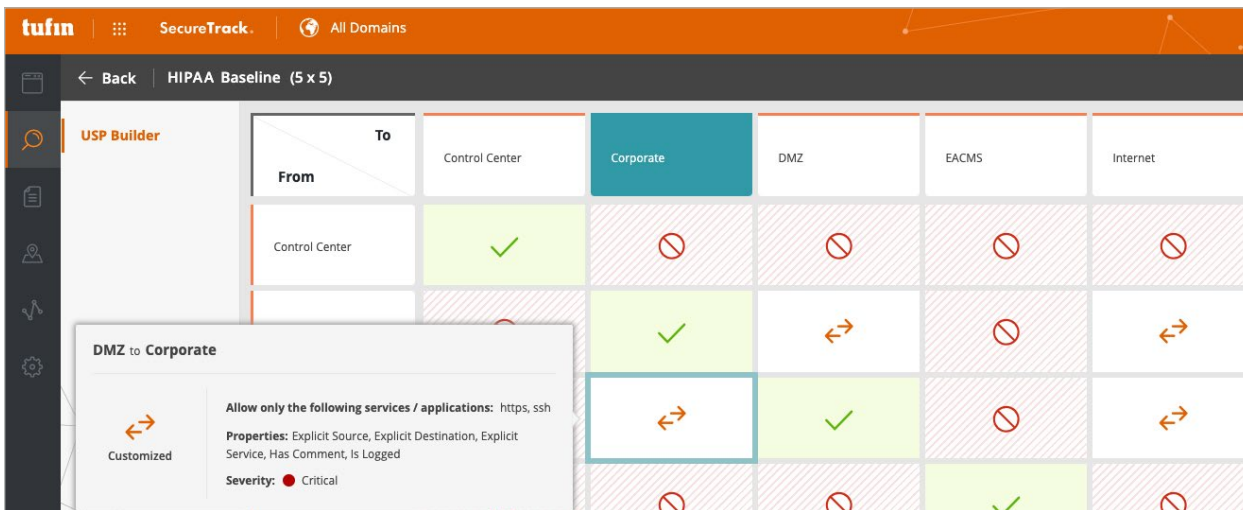
Enforcing HIPAA compliance with Tufin’s enterprise-wide Unified Security Policy zone matrix
